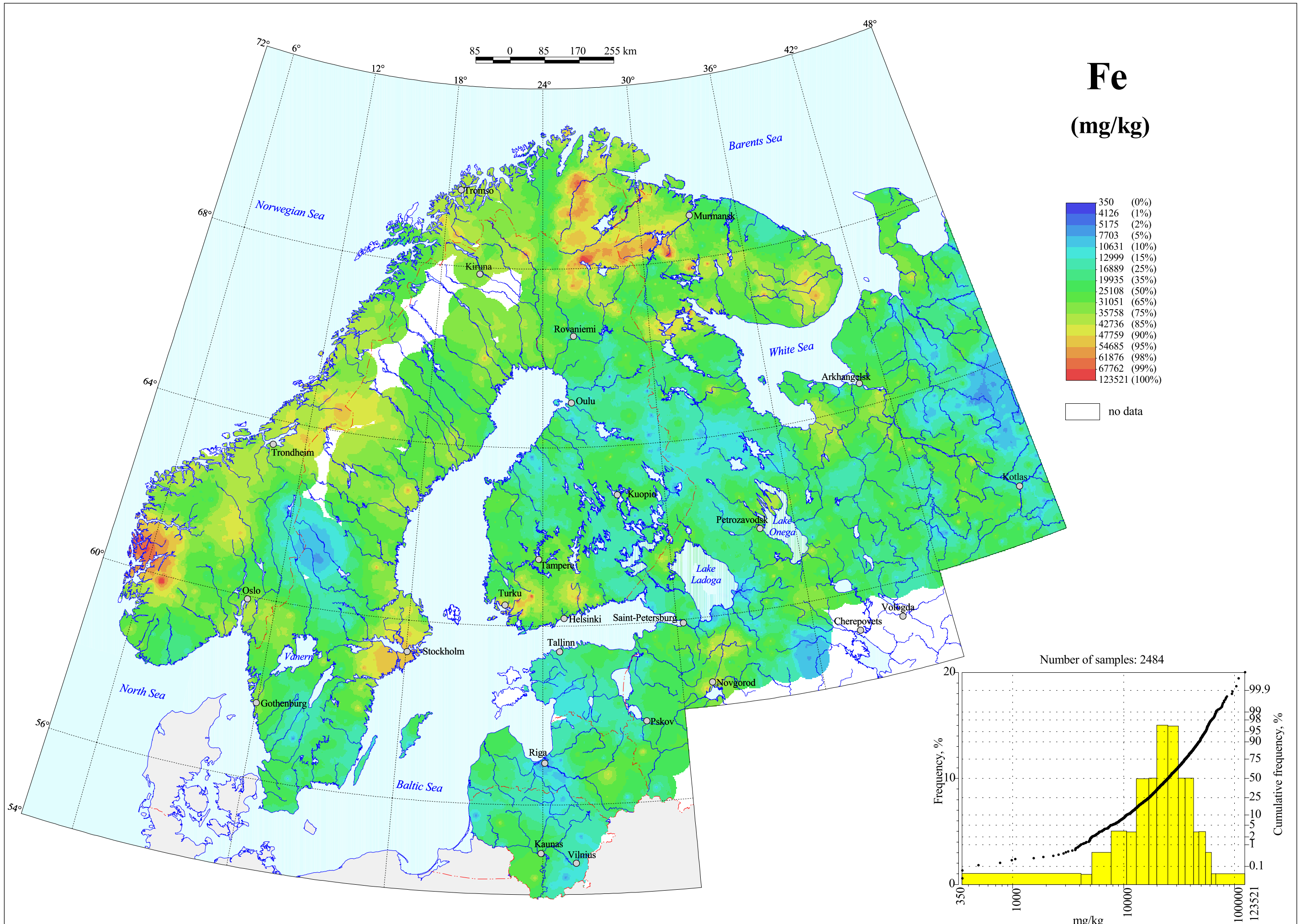
Iron in C-horizon, Grain Size <2 mm, Total Content
